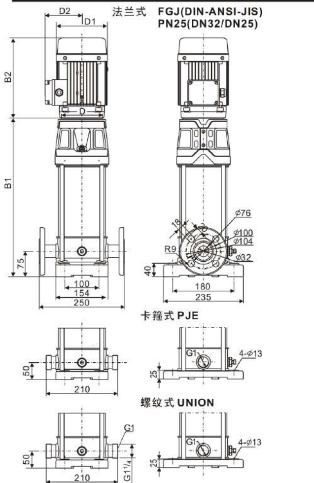
安装图/Installation sketch
